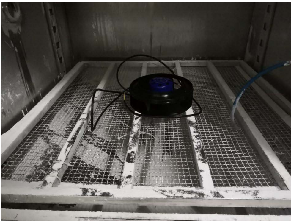
Sample setup-IP5X
